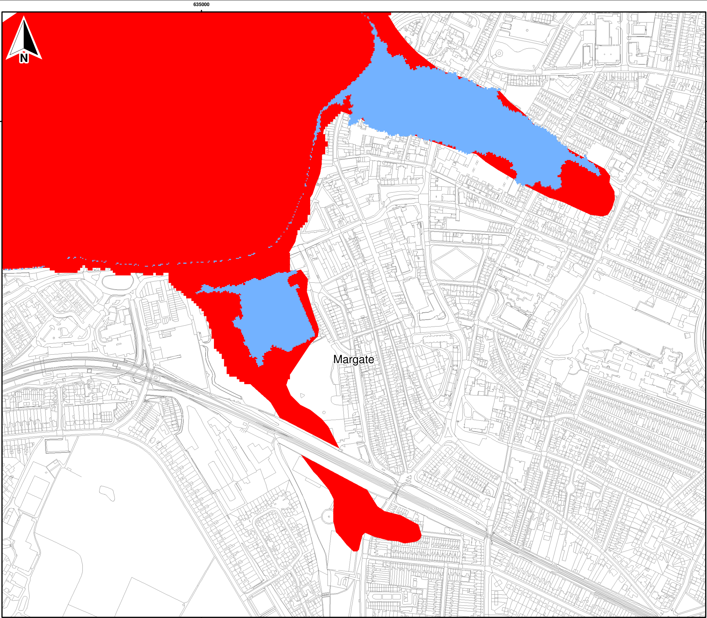
Thanet District SFRA Figure 7 Environment Agency Flood Zone 2 and Modelled undefended 1:1000 year tidal event (present day)
