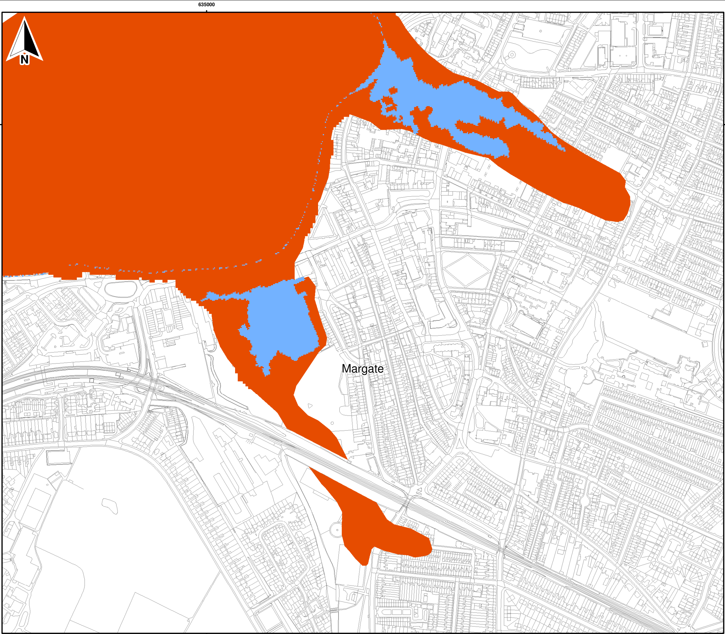
Thanet District SFRA Figure 8 Environment Agency Flood Zone 3 and Modelled undefended 1:200 year tidal event (present day)
