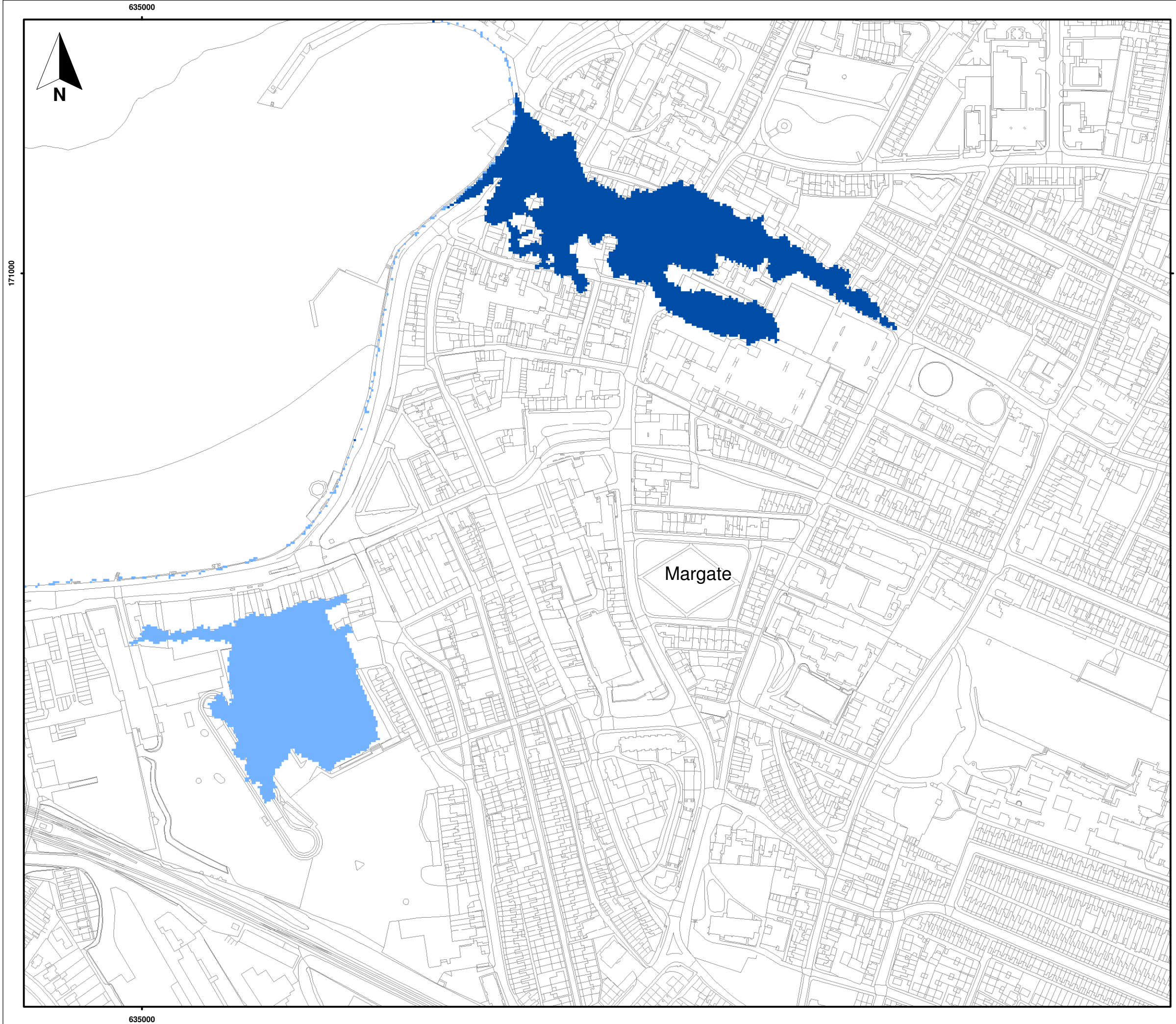
Figure 9 Residual Flood Risk Modelled event - 1 in 200 year
