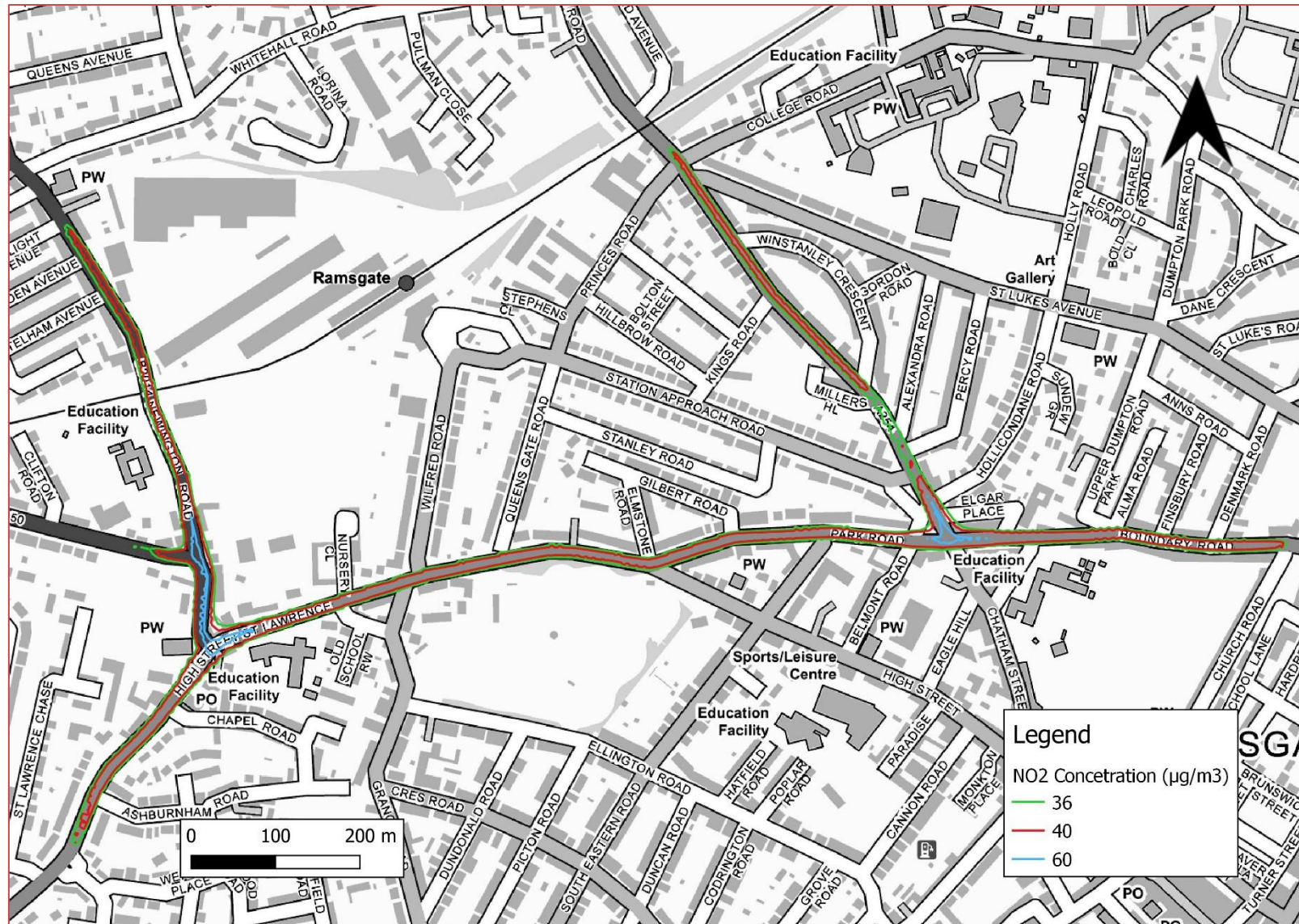
Figure 3.4 – St Lawrence, High Street, Modelled NO 2 Concentration Isopleths
